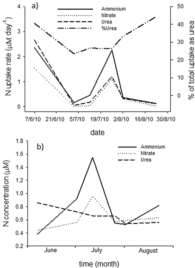
Fig. 5. a) The rate of uptake of ammonium, nitrate, and urea along with the percentage of total N uptake that was urea, in Loch Creran, Scotland, in summer 2010 determined by 15 N uptake. b) The concentrations of ammonium, nitrate and urea at the same (10 m) depth that the uptake experiments were conducted.
