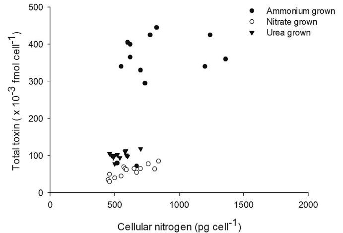
Fig. 6. The relationship between cellular N content and total toxin for Alexandrium tamarense grown separately on ammonium, nitrate and urea (redrawn from Leong et al., 2004).
