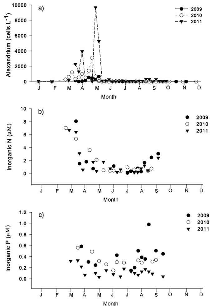
Fig. 1. Time course of: a) potentially harmful (saxitoxin producing) Alexandrium sp. cell abundance b) inorganic N and c) inorganic P in Loch Creran Scotland during the summers of 2009–2011.
